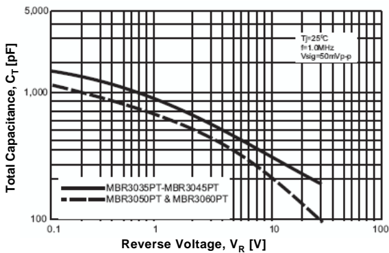
Figure 5. Total Capacitance
